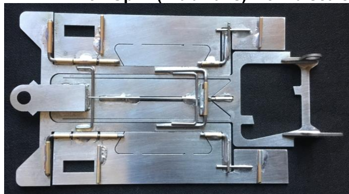
Betta Gp12 (Clubmans).
