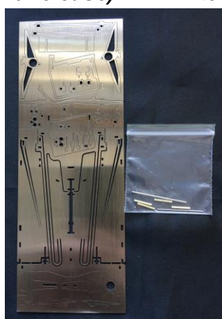
Mack Pro-Am sports kit
